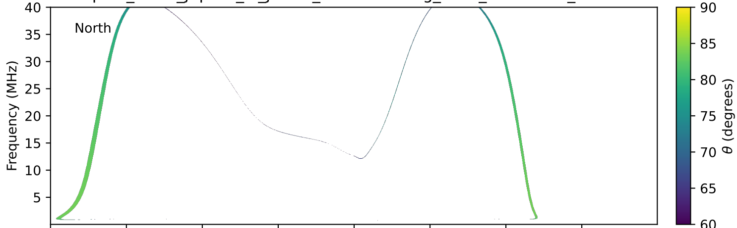
expres_earth_jupiter_io_jrm09_lossc-wid1deg_3kev_19940612_v11.cdf
