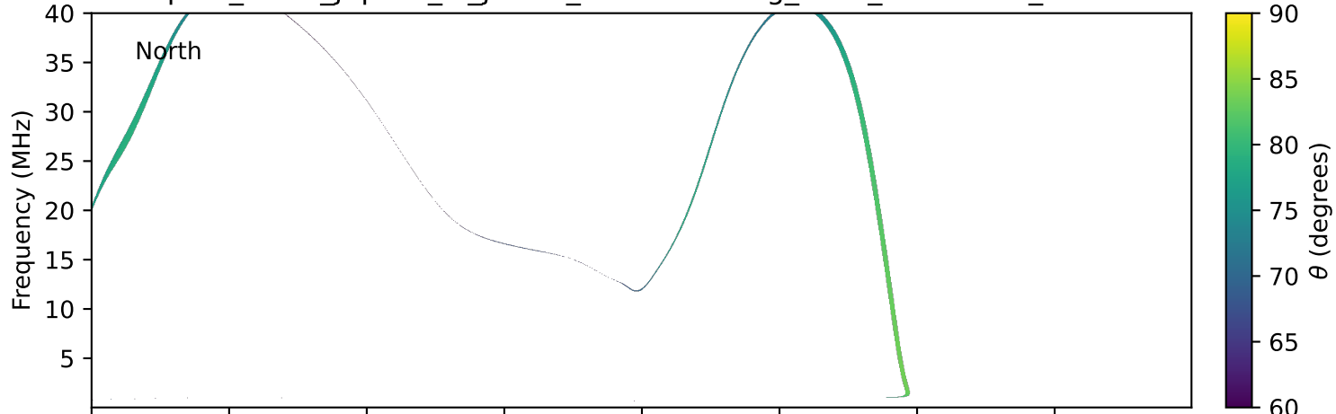
expres_earth_jupiter_io_jrm09_lossc-wid1deg_3kev_19940605_v11.cdf
