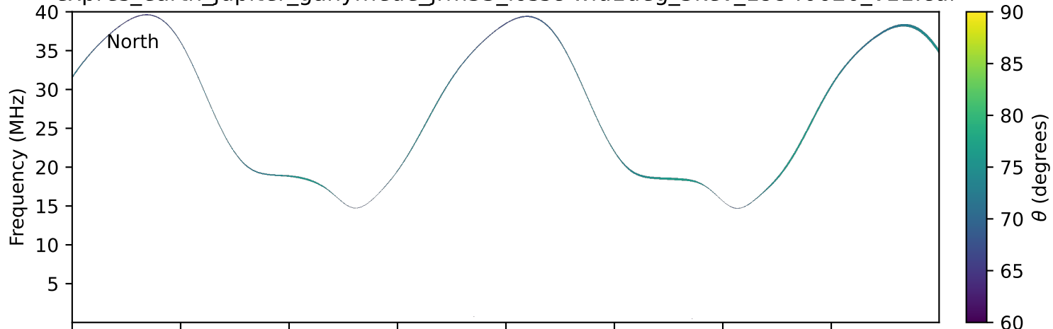
expres_earth_jupiter_ganymede_jrm33_lossc-wid1deg_3kev_19940620_v11.cdf
