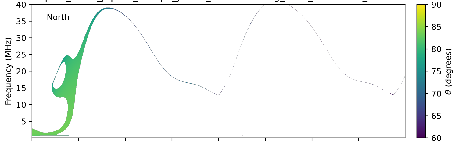
expres_earth_jupiter_europa_jrm09_lossc-wid1deg_3kev_19880105_v11.cdf
