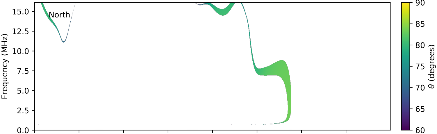
expres_cassini_jupiter_io_isaac_lossc-wid1deg_3kev_20031231_v01.cdf
