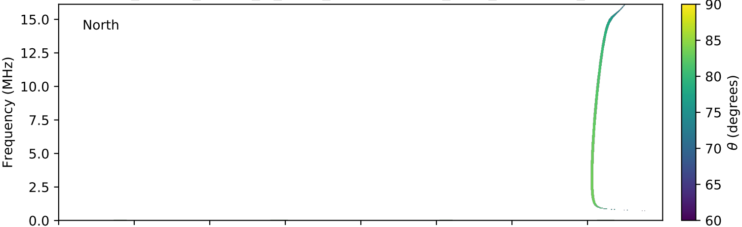
expres_cassini_jupiter_io_isaac_lossc-wid1deg_3kev_20031230_v01.cdf
