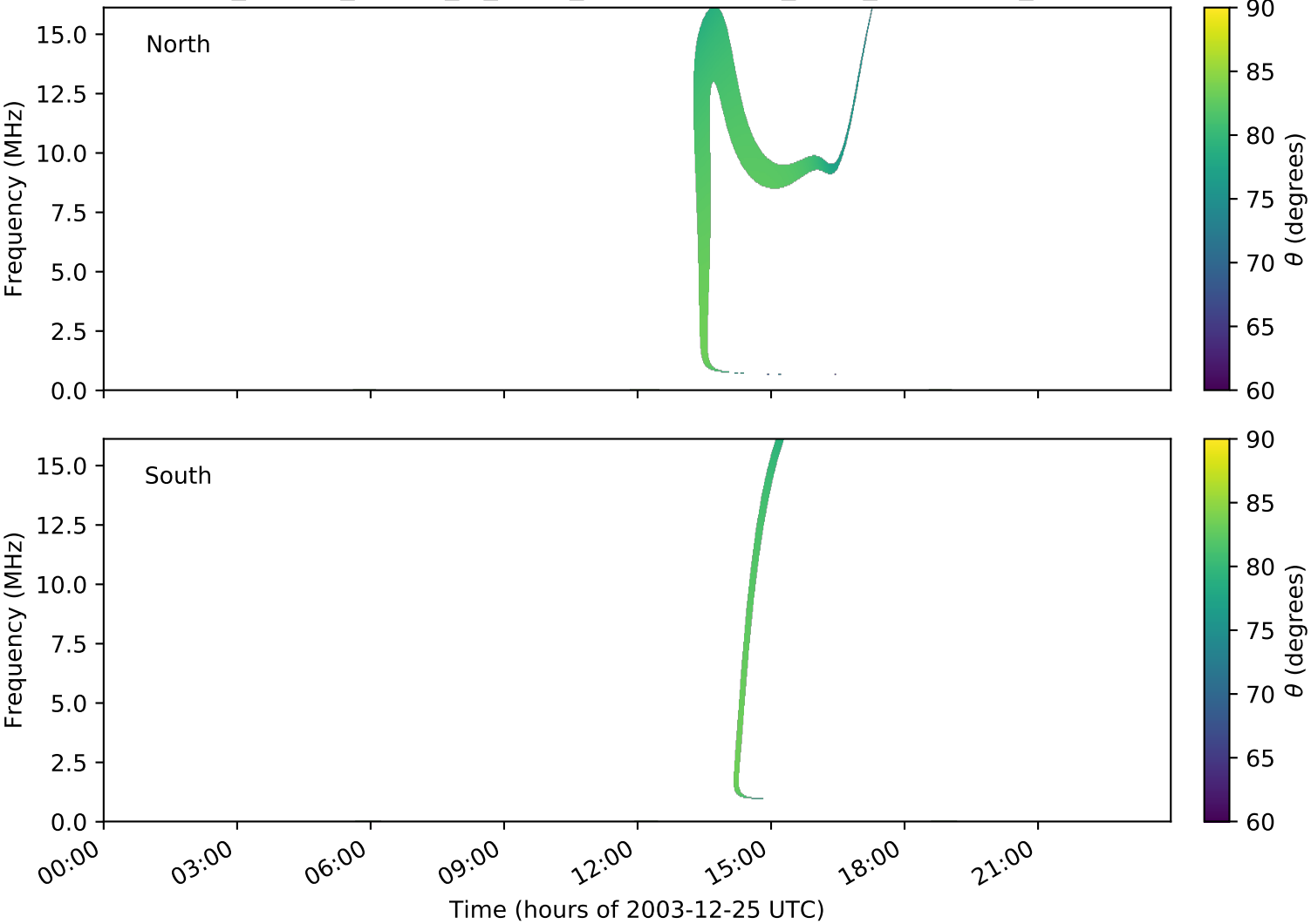
expres_cassini_jupiter_io_isaac_lossc-wid1deg_3kev_20031225_v01.cdf
