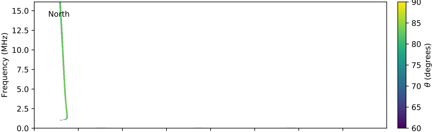
expres_cassini_jupiter_io_isaac_lossc-wid1deg_3kev_20031221_v01.cdf
