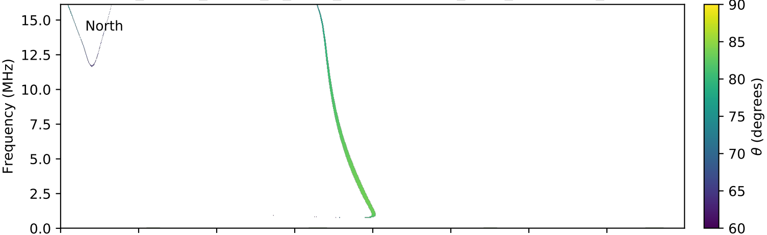
expres_cassini_jupiter_io_isaac_lossc-wid1deg_3kev_20031217_v01.cdf
