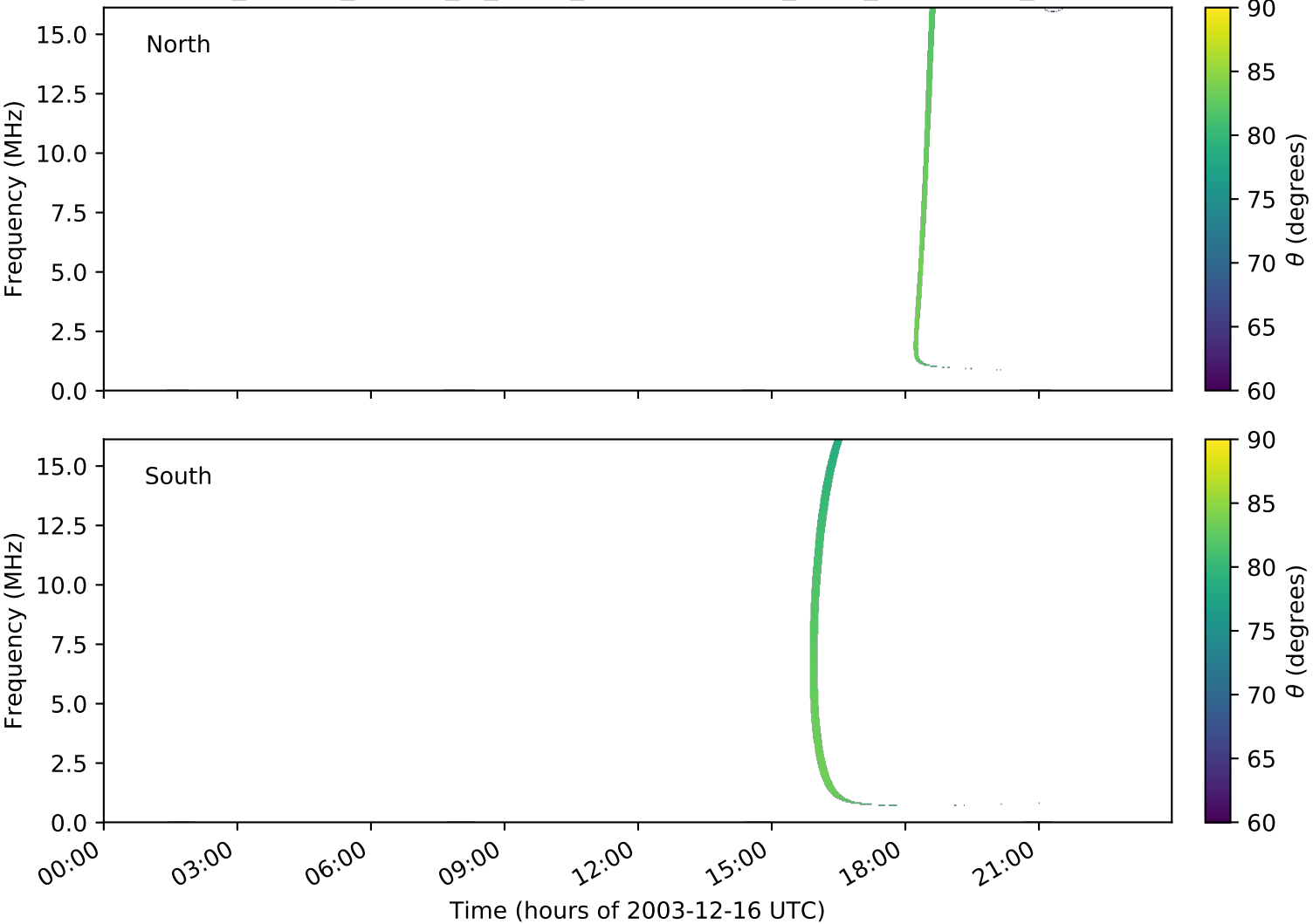
expres_cassini_jupiter_io_isaac_lossc-wid1deg_3kev_20031216_v01.cdf
