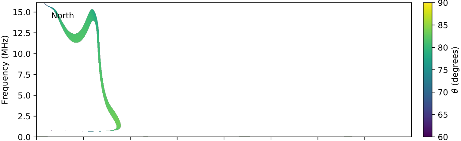
expres_cassini_jupiter_io_isaac_lossc-wid1deg_3kev_20031212_v01.cdf
