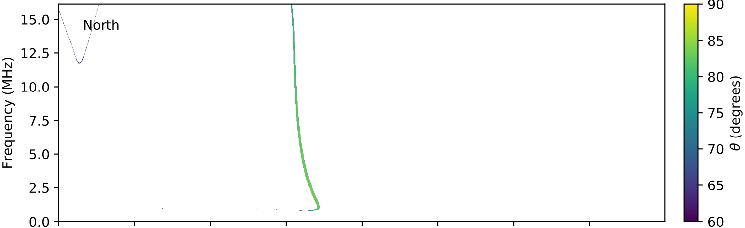
expres_cassini_jupiter_io_isaac_lossc-wid1deg_3kev_20031210_v01.cdf
