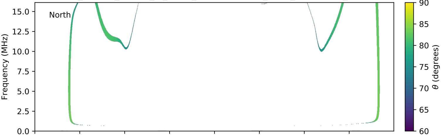
expres_cassini_jupiter_io_isaac_lossc-wid1deg_3kev_20031206_v01.cdf
