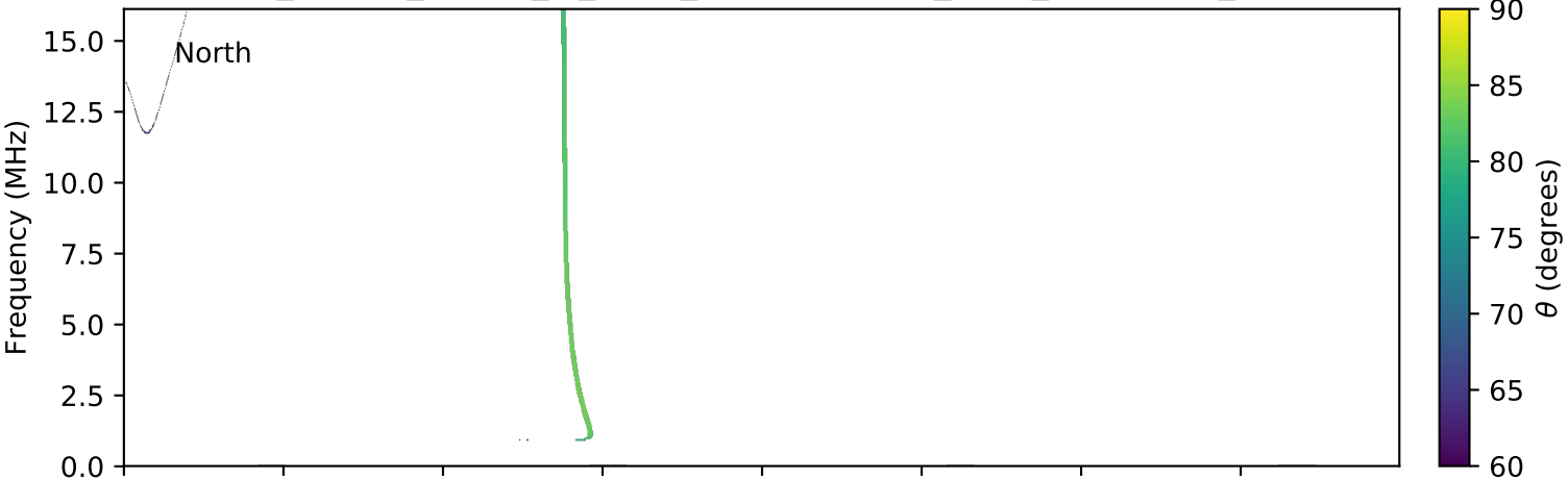
expres_cassini_jupiter_io_isaac_lossc-wid1deg_3kev_20031203_v01.cdf
