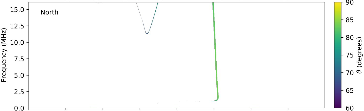
expres_cassini_jupiter_io_isaac_lossc-wid1deg_3kev_20031201_v01.cdf
