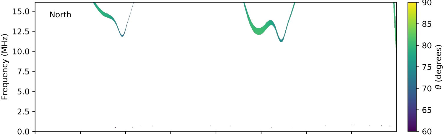
expres_cassini_jupiter_ganymede_isaac_lossc-wid1deg_3kev_20031228_v01.cdf
