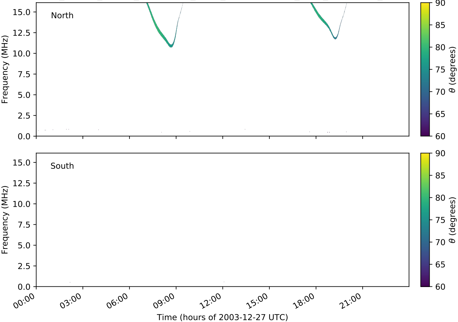
expres_cassini_jupiter_ganymede_isaac_lossc-wid1deg_3kev_20031227_v01.cdf
