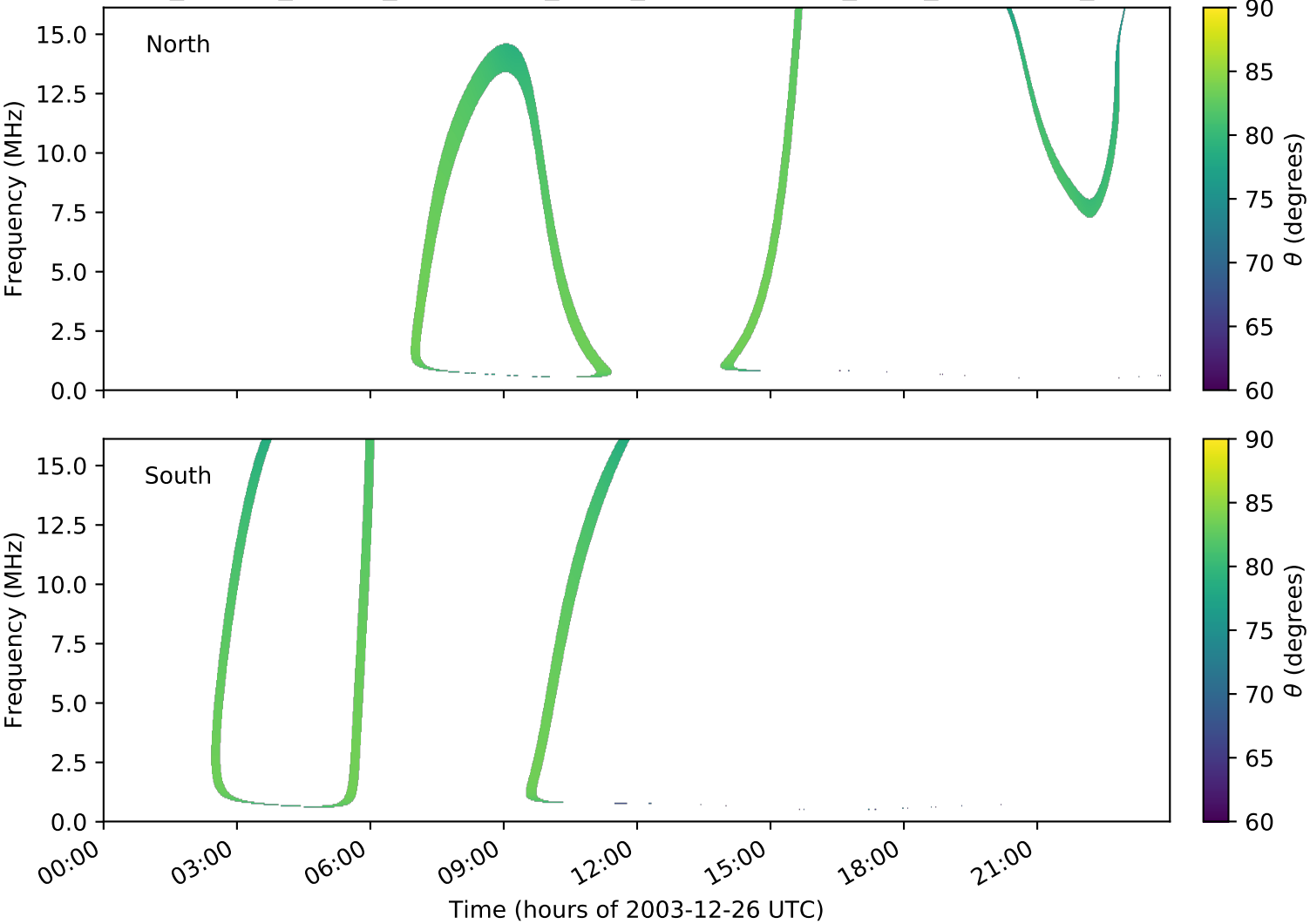
expres_cassini_jupiter_ganymede_isaac_lossc-wid1deg_3kev_20031226_v01.cdf
