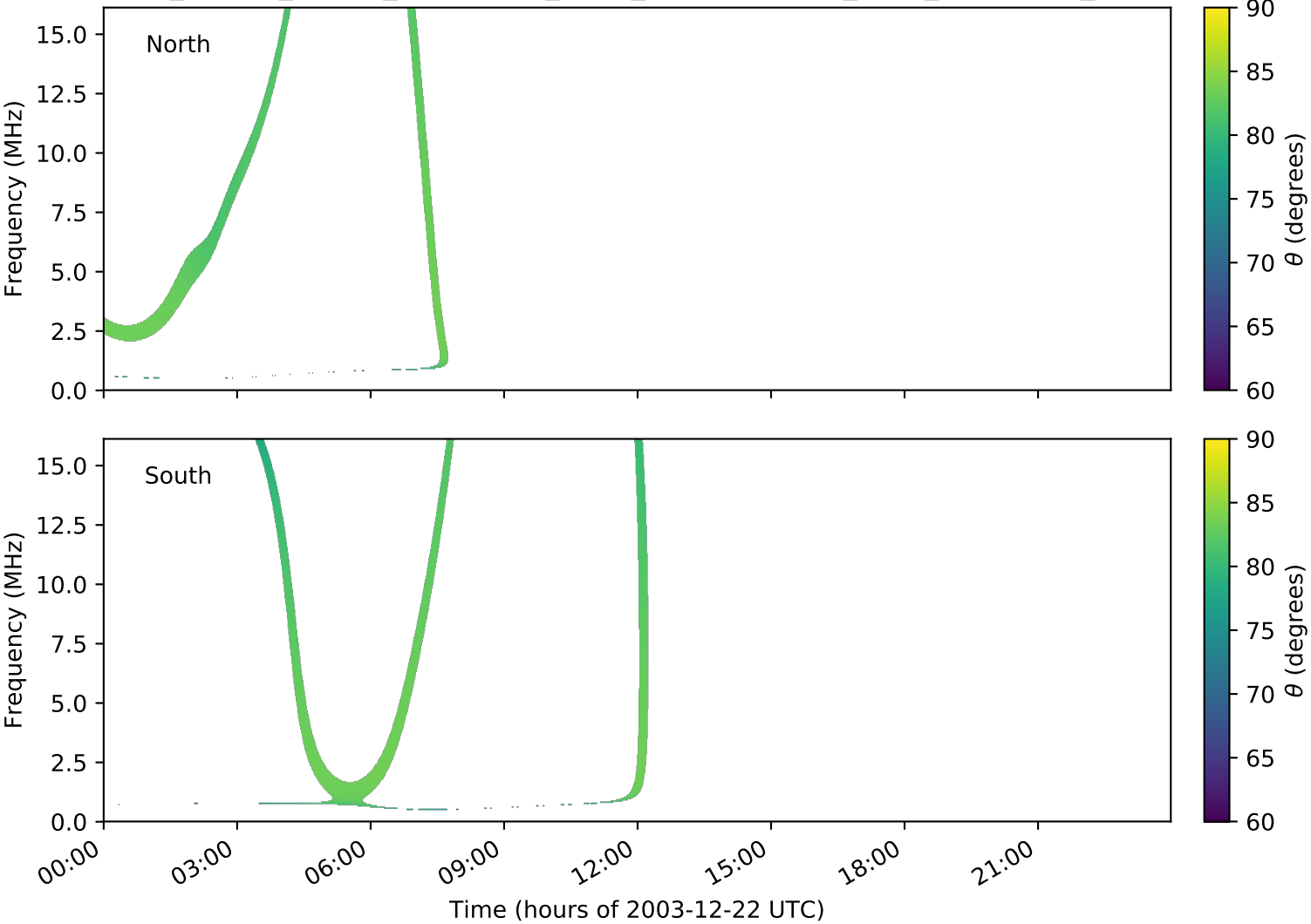
expres_cassini_jupiter_ganymede_isaac_lossc-wid1deg_3kev_20031222_v01.cdf
