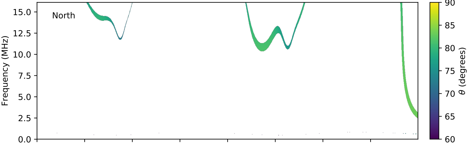
expres_cassini_jupiter_ganymede_isaac_lossc-wid1deg_3kev_20031221_v01.cdf
