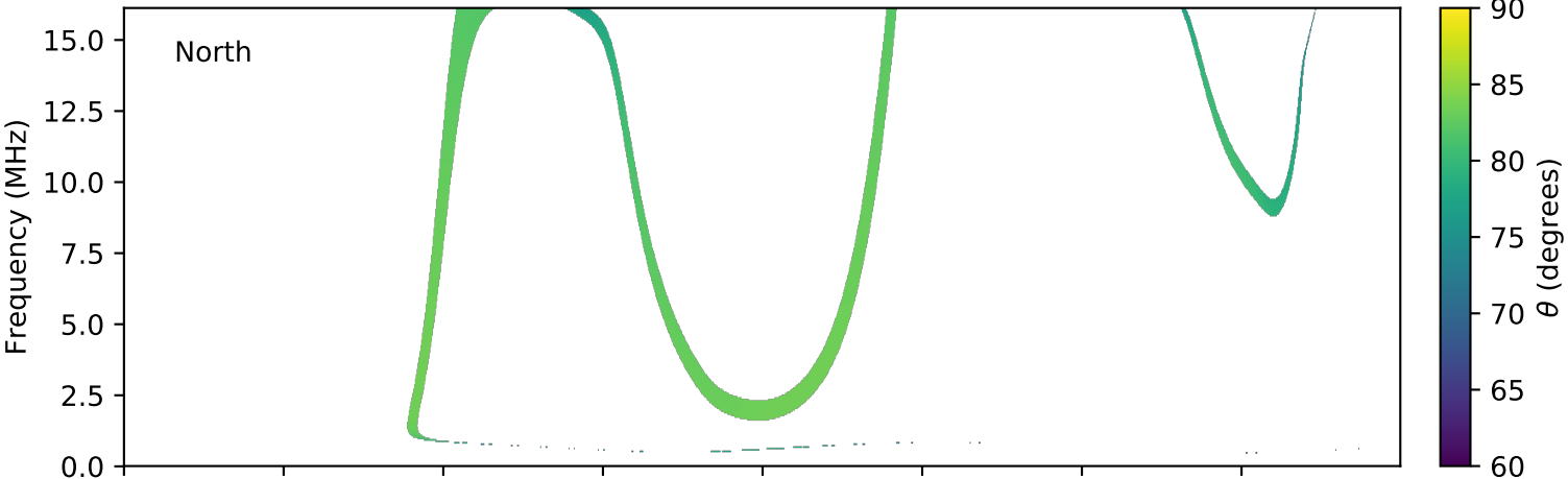
expres_cassini_jupiter_ganymede_isaac_lossc-wid1deg_3kev_20031219_v01.cdf
