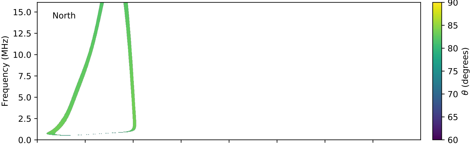
expres_cassini_jupiter_ganymede_isaac_lossc-wid1deg_3kev_20031215_v01.cdf
