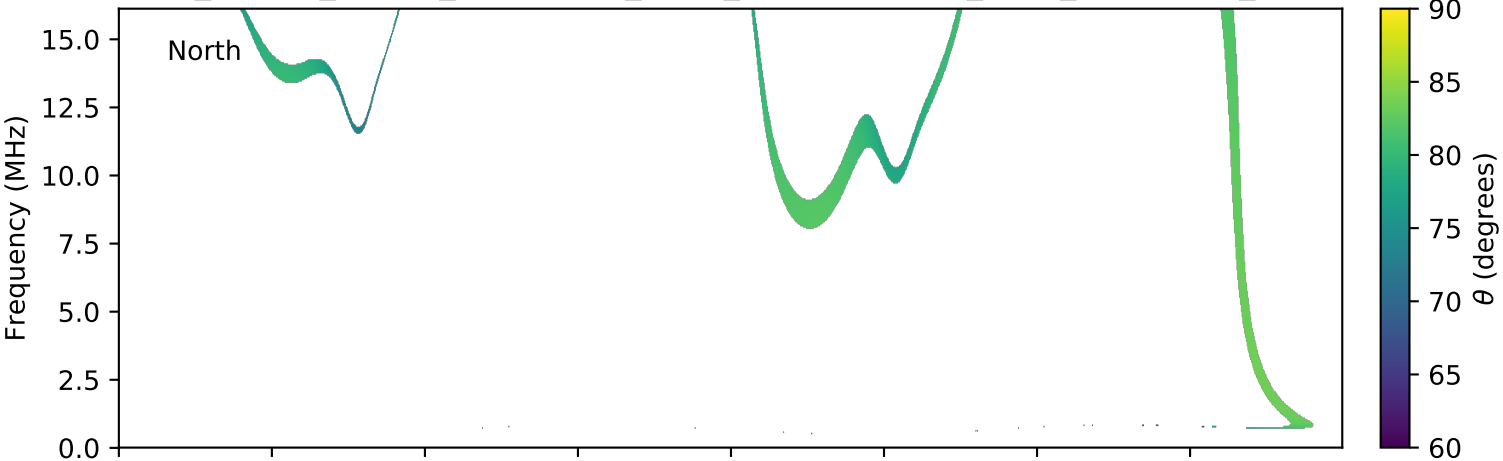
expres_cassini_jupiter_ganymede_isaac_lossc-wid1deg_3kev_20031214_v01.cdf
