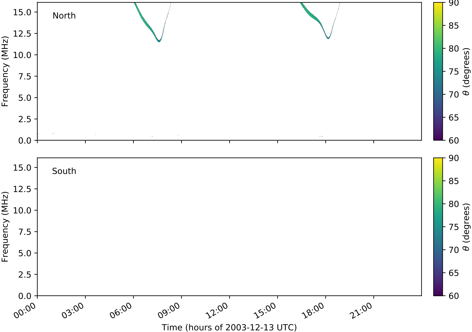
expres_cassini_jupiter_ganymede_isaac_lossc-wid1deg_3kev_20031213_v01.cdf
