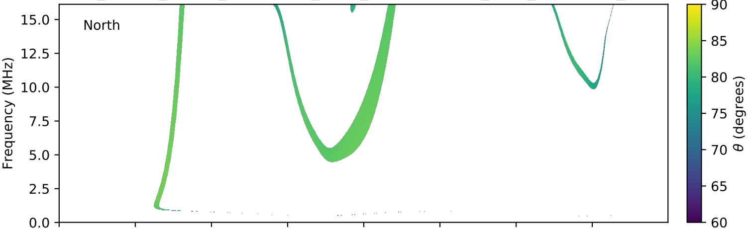
expres_cassini_jupiter_ganymede_isaac_lossc-wid1deg_3kev_20031212_v01.cdf
