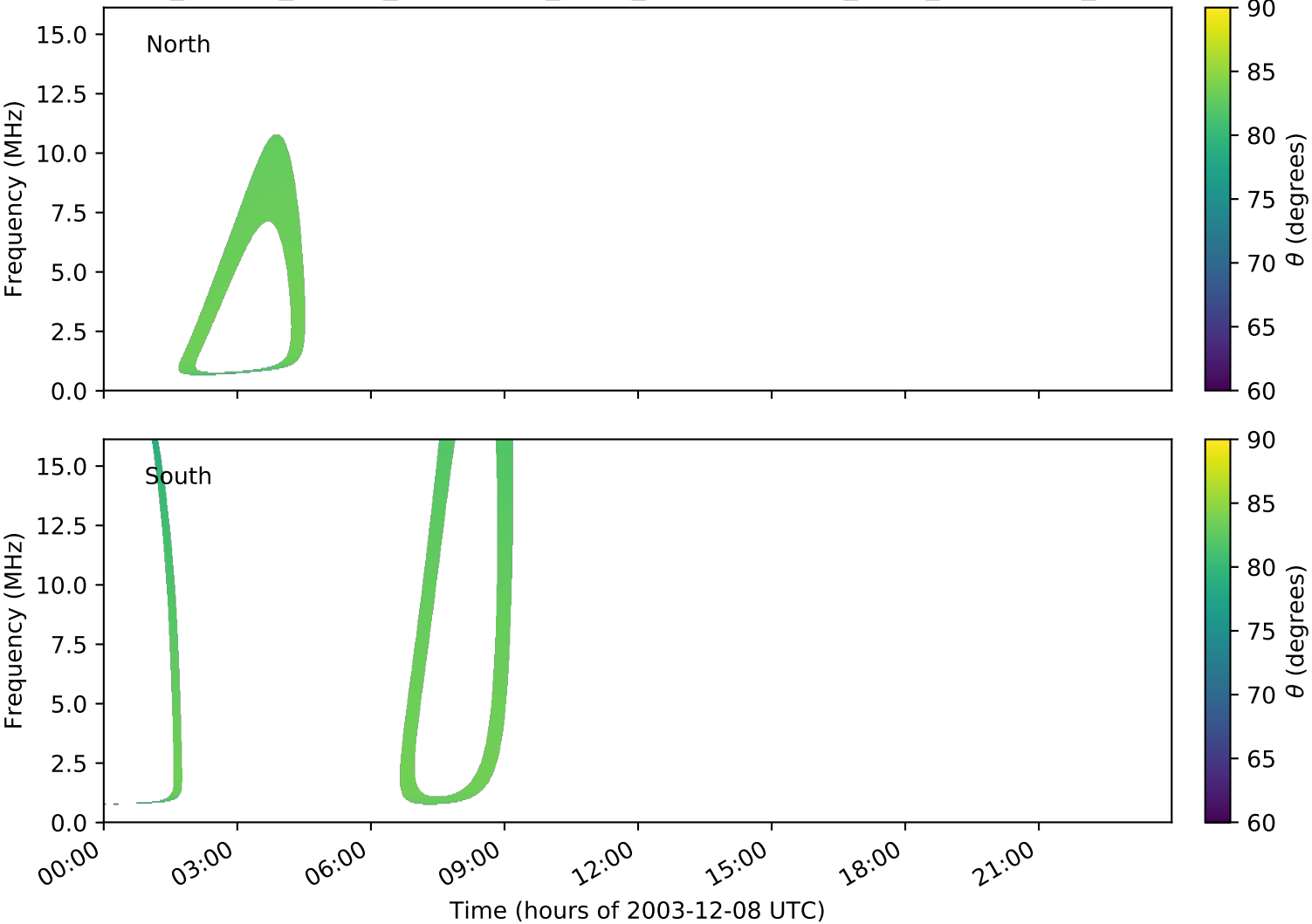
expres_cassini_jupiter_ganymede_isaac_lossc-wid1deg_3kev_20031208_v01.cdf
