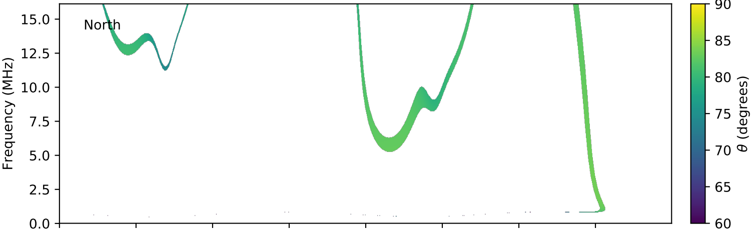
expres_cassini_jupiter_ganymede_isaac_lossc-wid1deg_3kev_20031207_v01.cdf
