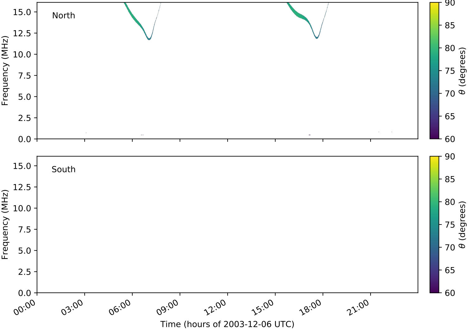
expres_cassini_jupiter_ganymede_isaac_lossc-wid1deg_3kev_20031206_v01.cdf
