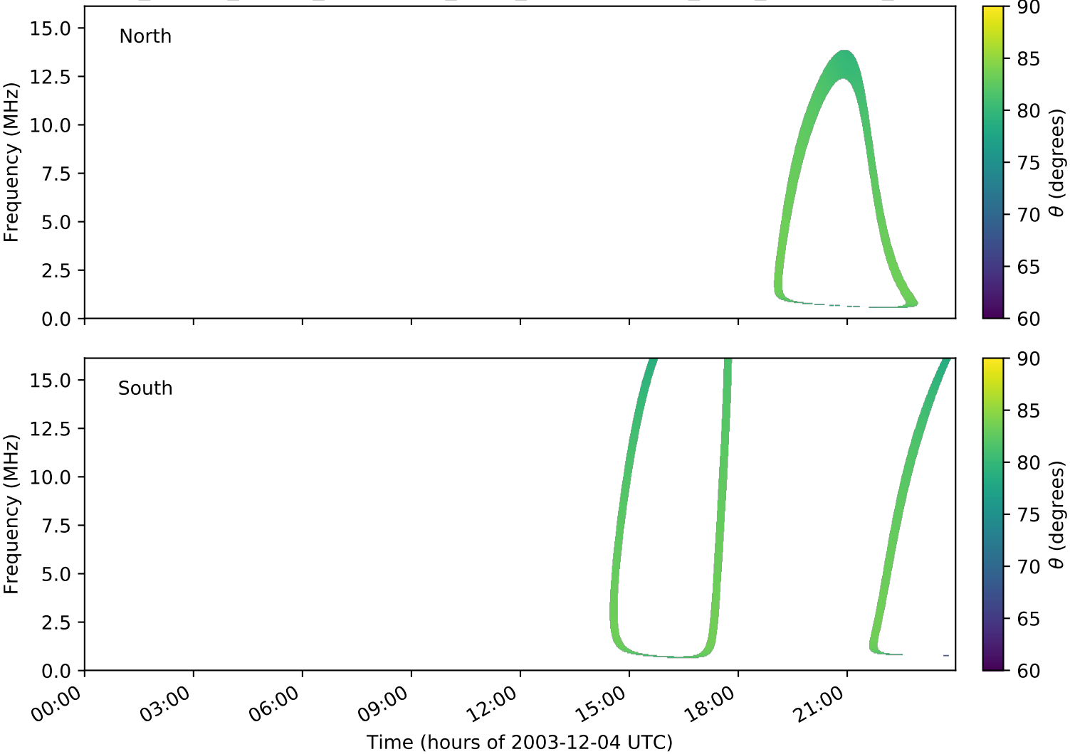
expres_cassini_jupiter_ganymede_isaac_lossc-wid1deg_3kev_20031204_v01.cdf
