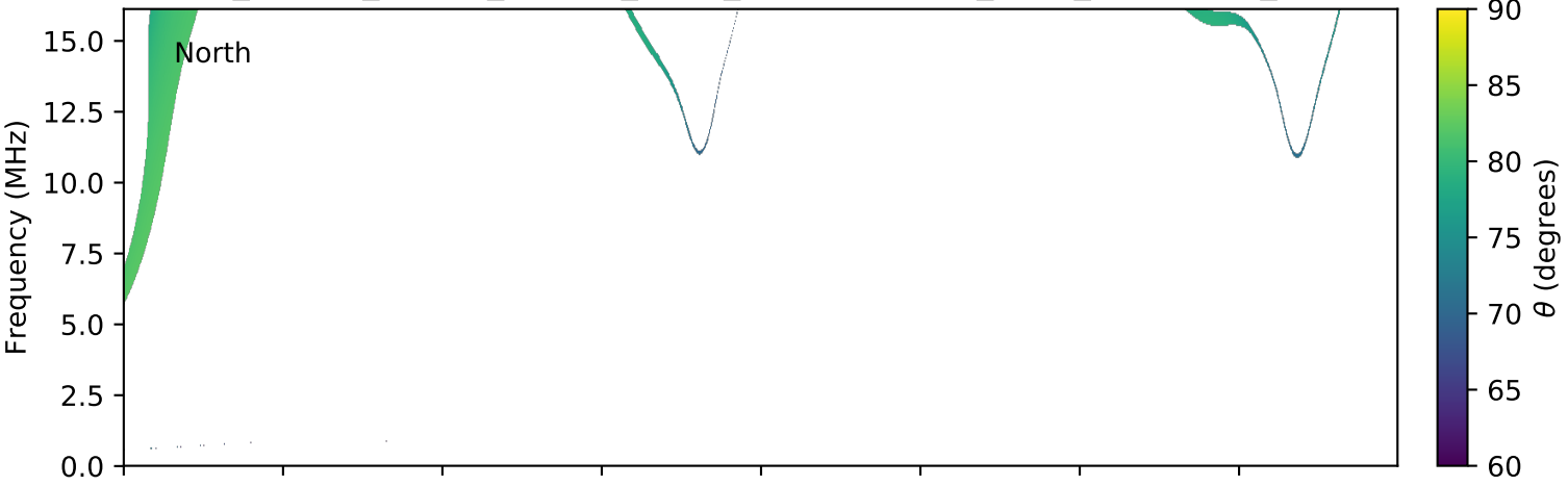
expres_cassini_jupiter_europa_isaac_lossc-wid1deg_3kev_20031229_v01.cdf
