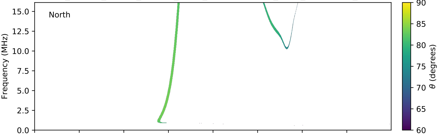
expres_cassini_jupiter_europa_isaac_lossc-wid1deg_3kev_20031225_v01.cdf
