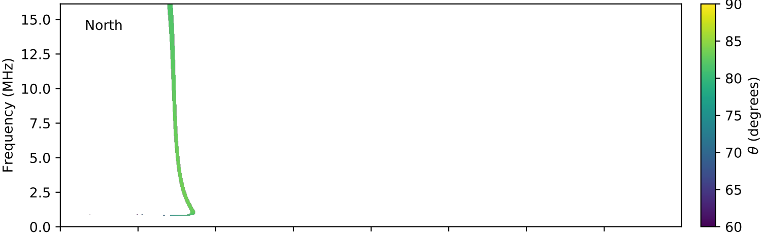
expres_cassini_jupiter_europa_isaac_lossc-wid1deg_3kev_20031223_v01.cdf
