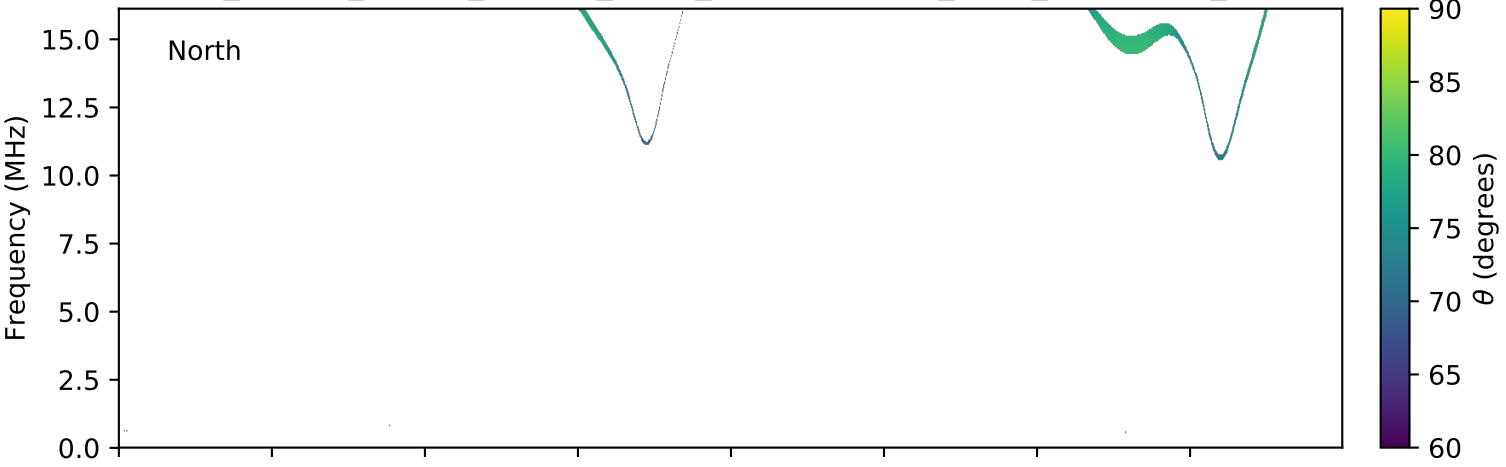
expres_cassini_jupiter_europa_isaac_lossc-wid1deg_3kev_20031222_v01.cdf
