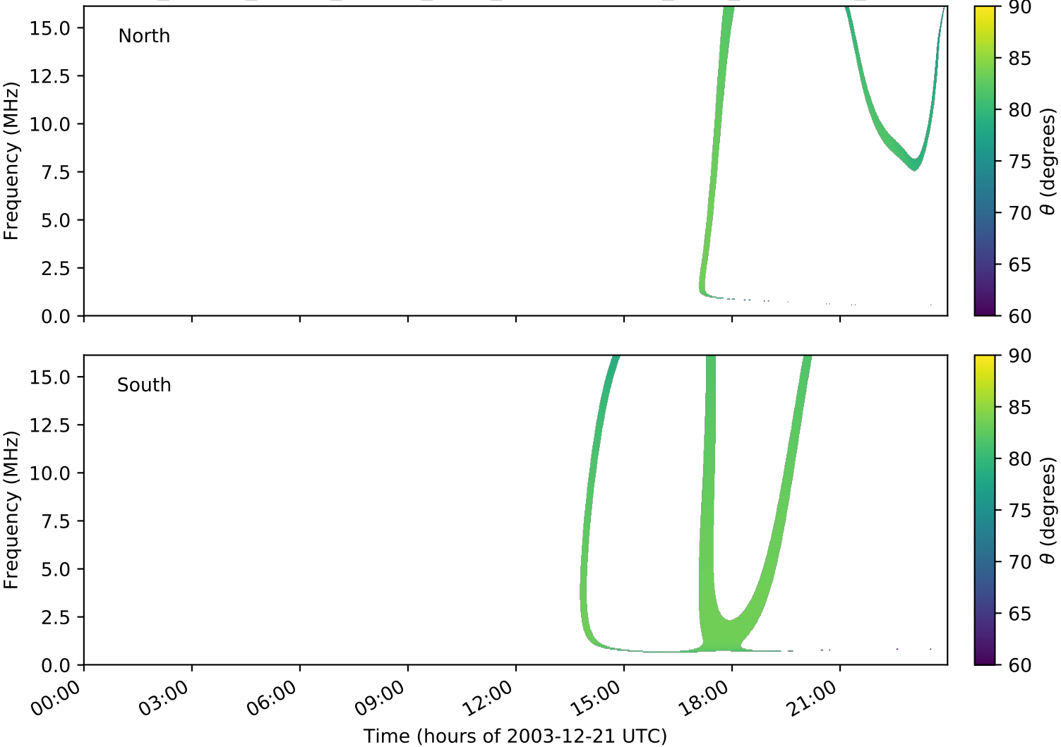
expres_cassini_jupiter_europa_isaac_lossc-wid1deg_3kev_20031221_v01.cdf
