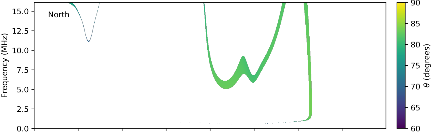
expres_cassini_jupiter_europa_isaac_lossc-wid1deg_3kev_20031219_v01.cdf
