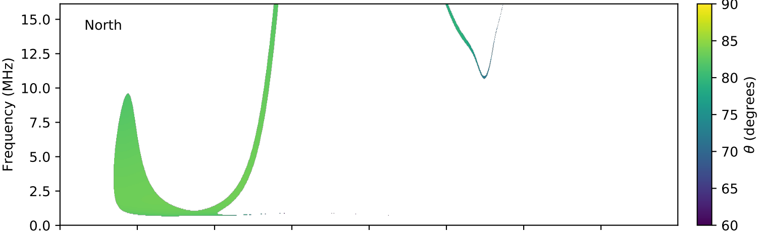
expres_cassini_jupiter_europa_isaac_lossc-wid1deg_3kev_20031218_v01.cdf
