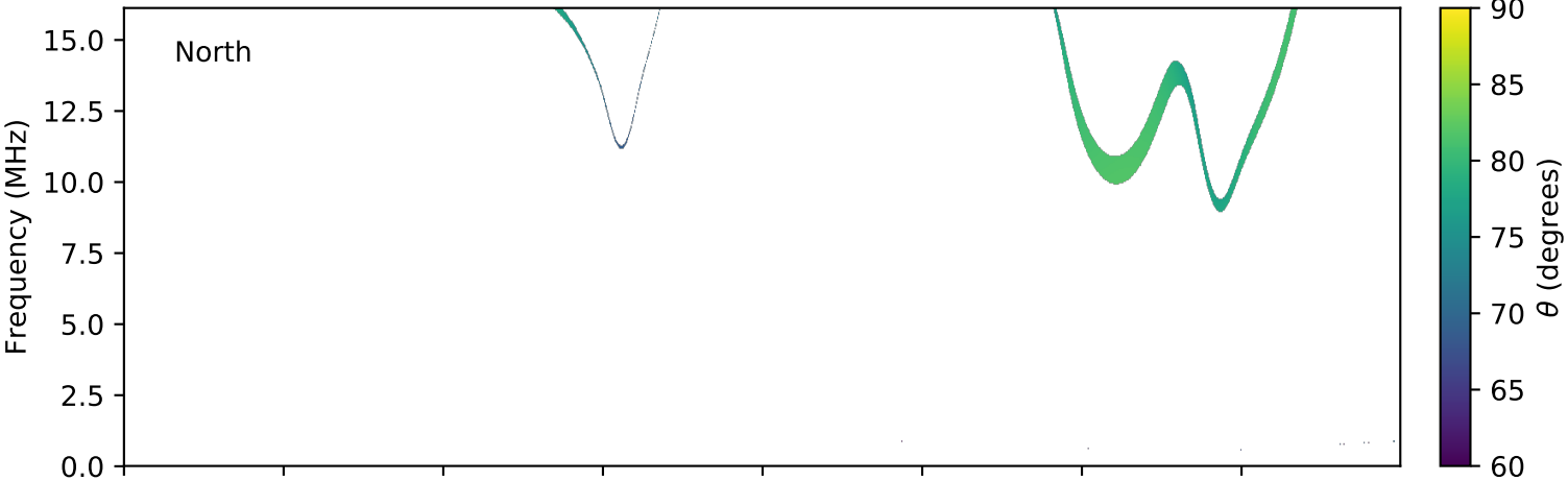
expres_cassini_jupiter_europa_isaac_lossc-wid1deg_3kev_20031208_v01.cdf
