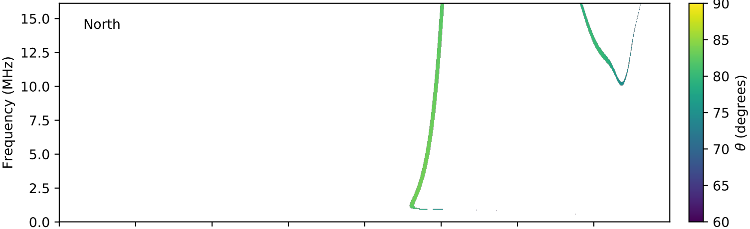
expres_cassini_jupiter_europa_isaac_lossc-wid1deg_3kev_20031207_v01.cdf
