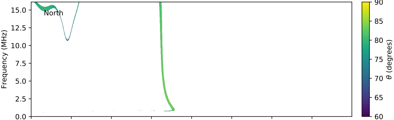
expres_cassini_jupiter_europa_isaac_lossc-wid1deg_3kev_20031205_v01.cdf
