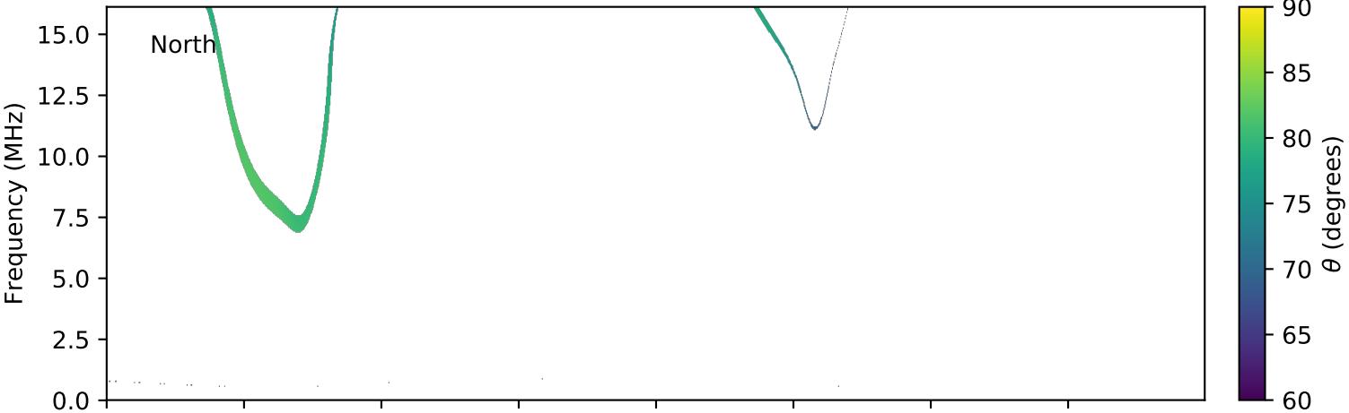
expres_cassini_jupiter_europa_isaac_lossc-wid1deg_3kev_20031204_v01.cdf
