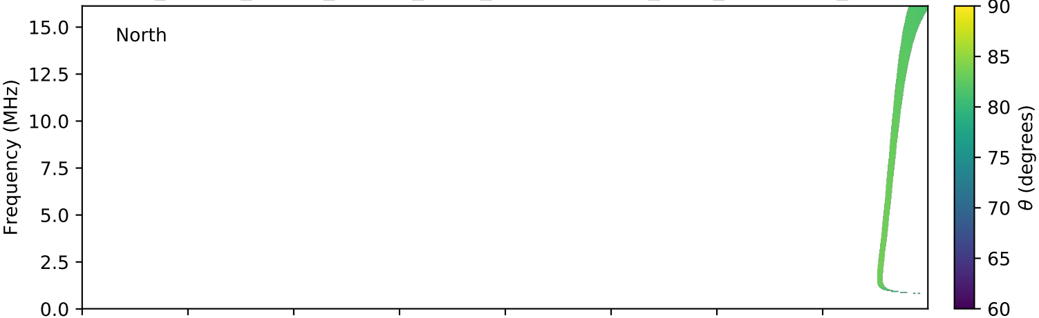
expres_cassini_jupiter_europa_isaac_lossc-wid1deg_3kev_20031203_v01.cdf
