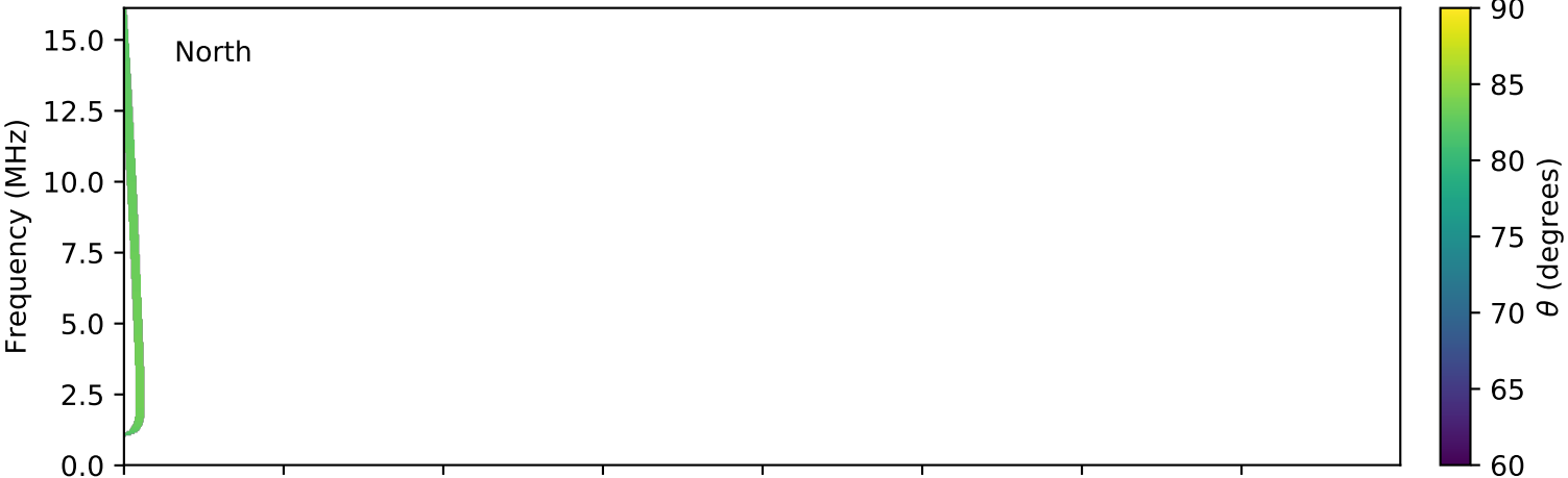
expres_cassini_jupiter_europa_isaac_lossc-wid1deg_3kev_20031202_v01.cdf
