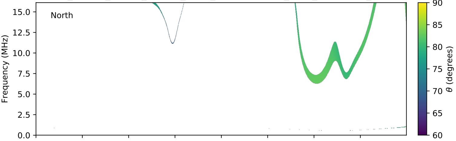
expres_cassini_jupiter_europa_isaac_lossc-wid1deg_3kev_20031201_v01.cdf
