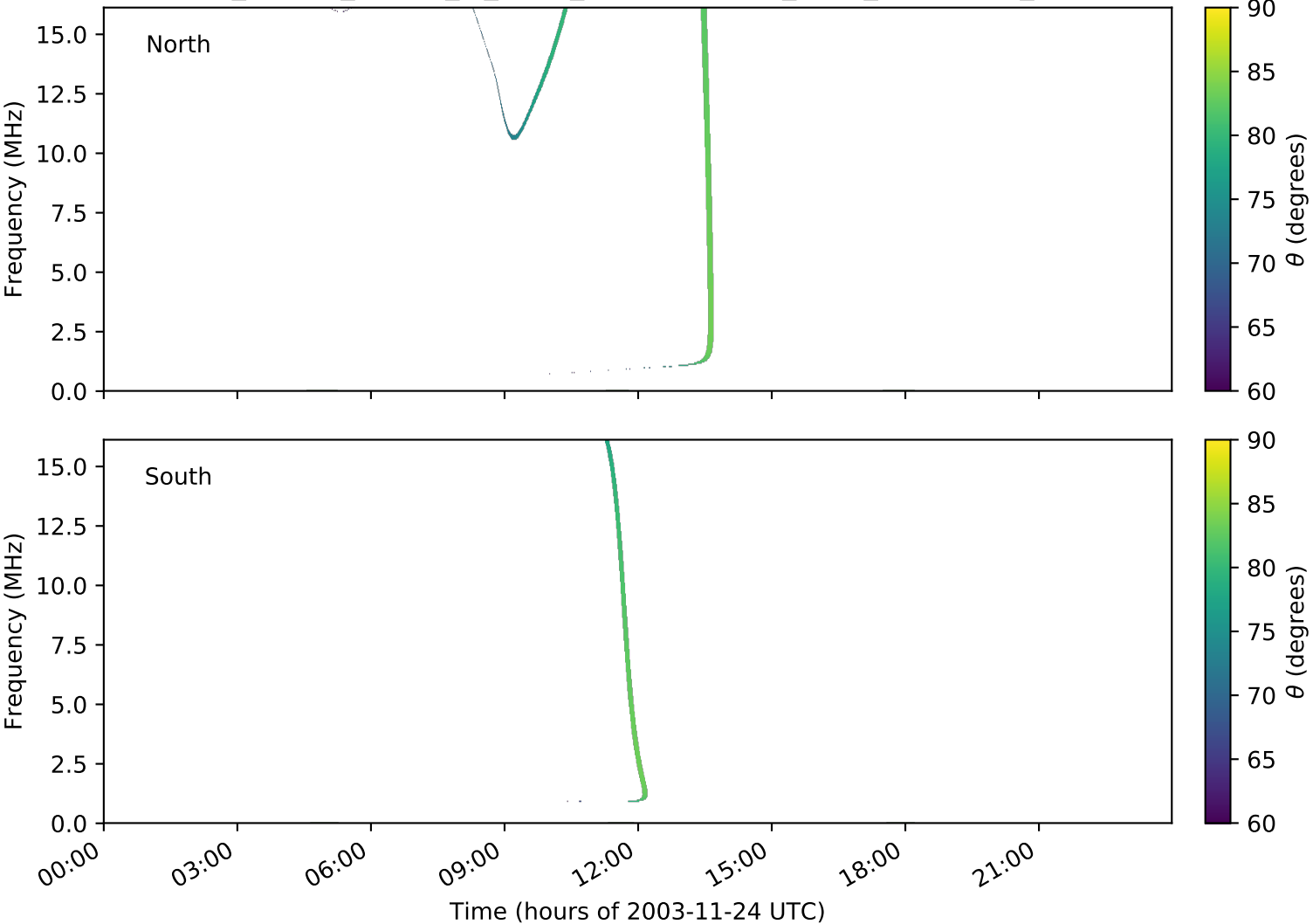
expres_cassini_jupiter_io_isaac_lossc-wid1deg_3kev_20031124_v01.cdf
