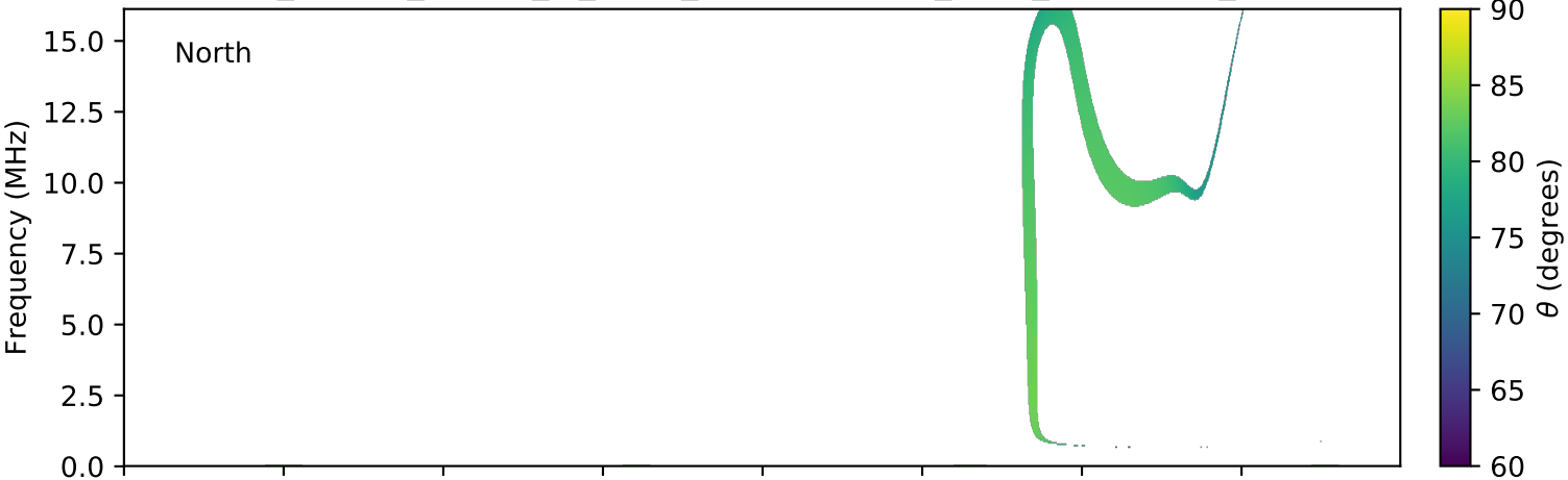
expres_cassini_jupiter_io_isaac_lossc-wid1deg_3kev_20031123_v01.cdf
