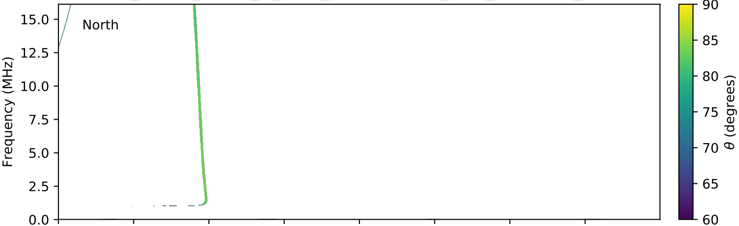
expres_cassini_jupiter_io_isaac_lossc-wid1deg_3kev_20031119_v01.cdf
