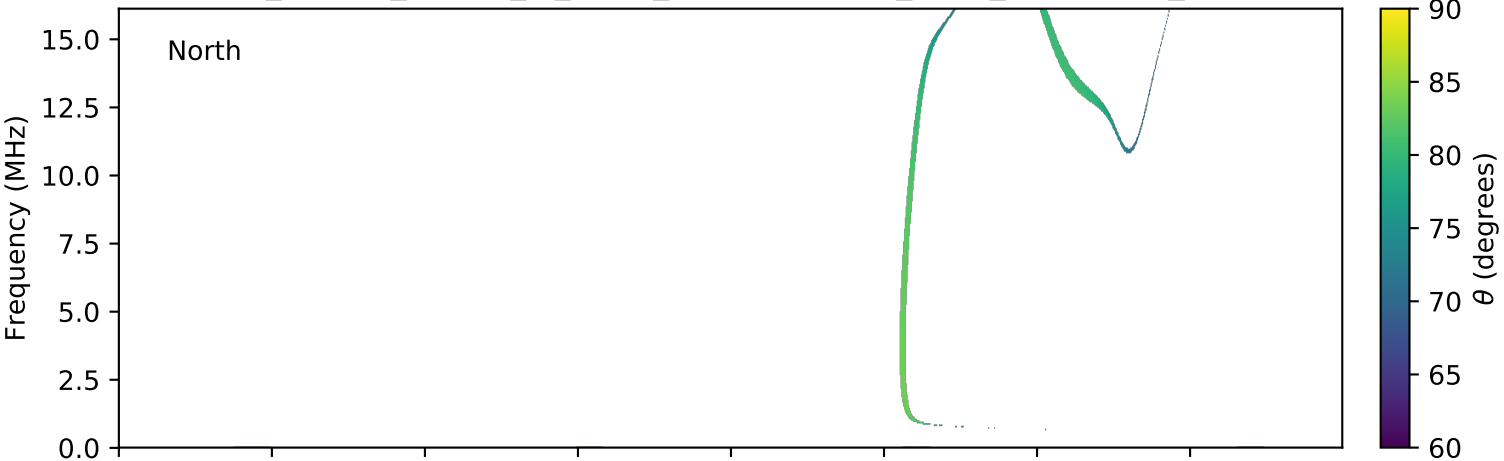
expres_cassini_jupiter_io_isaac_lossc-wid1deg_3kev_20031116_v01.cdf
