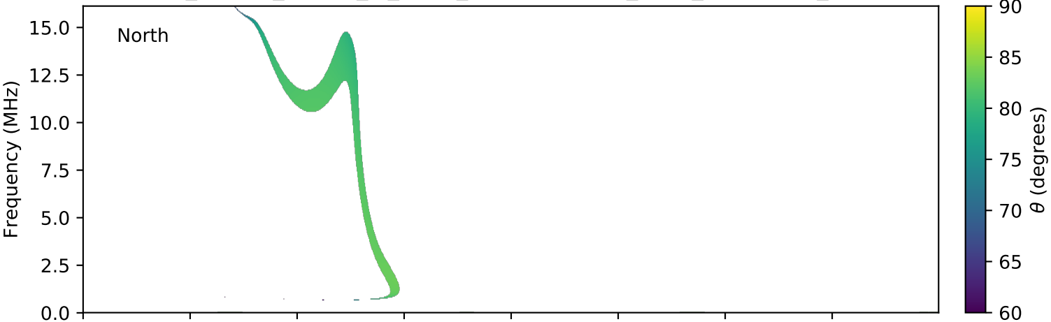
expres_cassini_jupiter_io_isaac_lossc-wid1deg_3kev_20031110_v01.cdf
