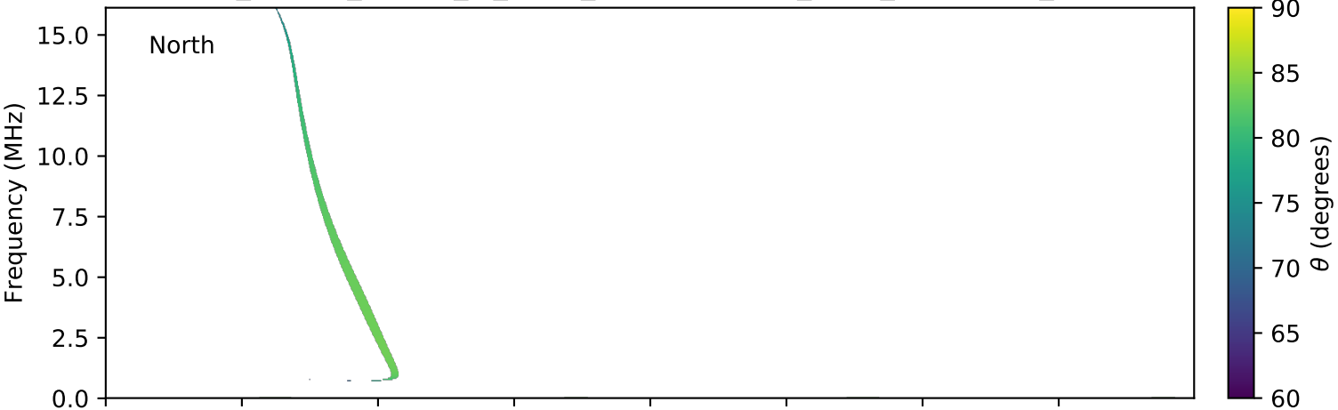
expres_cassini_jupiter_io_isaac_lossc-wid1deg_3kev_20031103_v01.cdf
