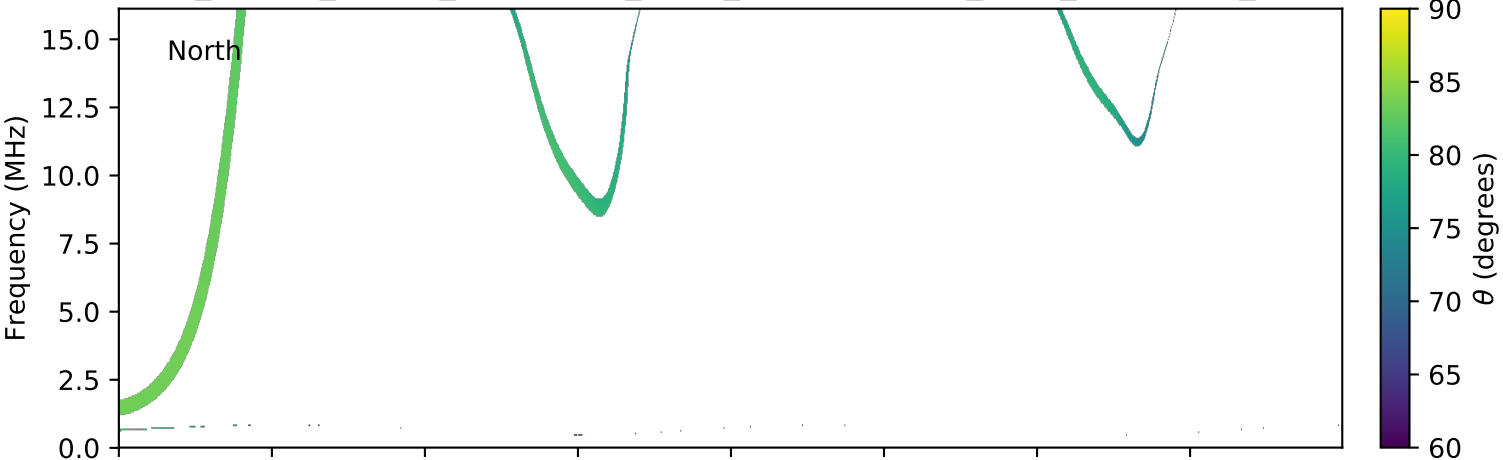
expres_cassini_jupiter_ganymede_isaac_lossc-wid1deg_3kev_20031128_v01.cdf
